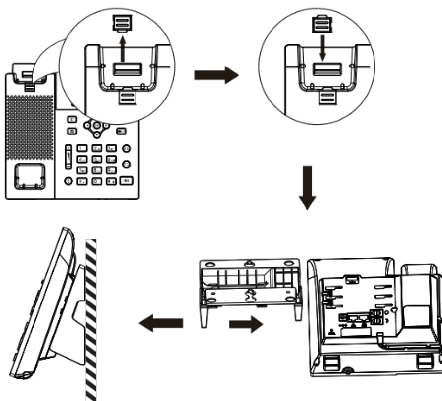
Picture 2 - Desktop to wall-mounted
